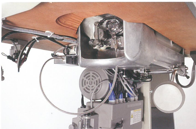
for horizontal-axis hook
